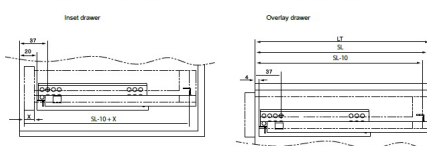
Installation dimensions
